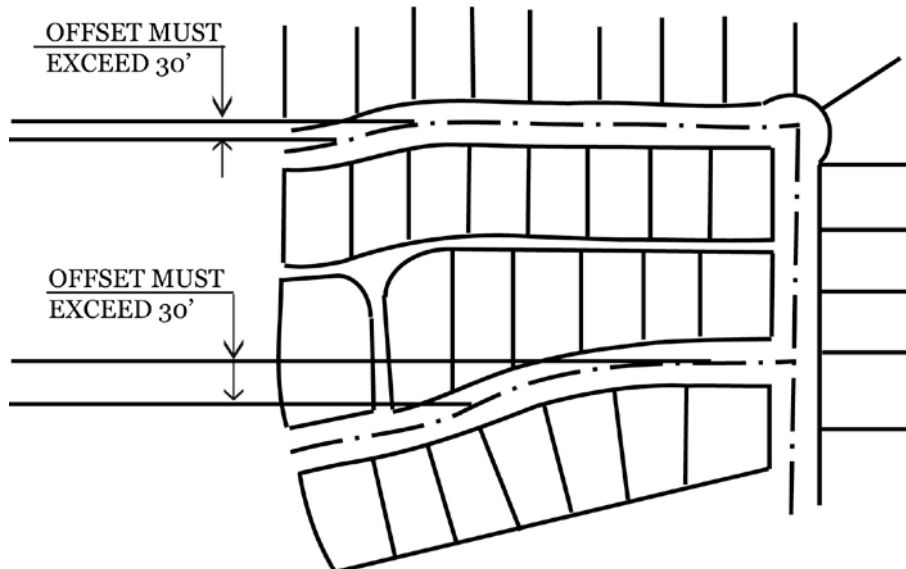
Figure 9-2: Curvilinear Streets
