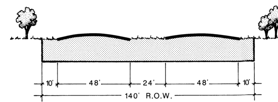
Type B+ (M8DA) Arterial - Regional With 12' Access Lanes
