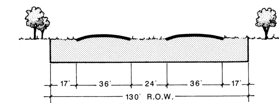
Type B (M6DA) Arterial - Regional
