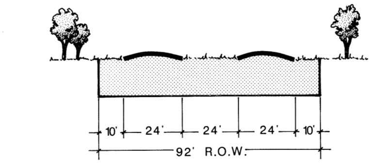
Type D (S4D) Secondary Thoroughfare
