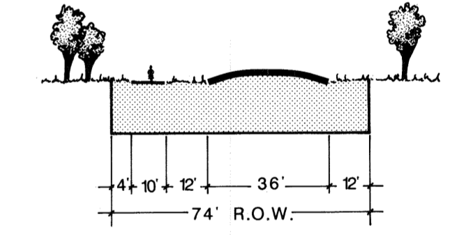
Type F (S2UI) Collector With Bike Path
