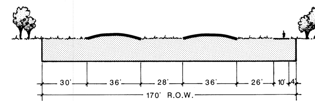
Type A (E6DAI) Arterial - Regional Limited Access With Bike Path
