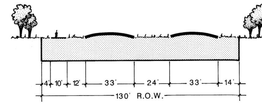
Type C (M6DI) Major Thoroughfare With Bike Path
