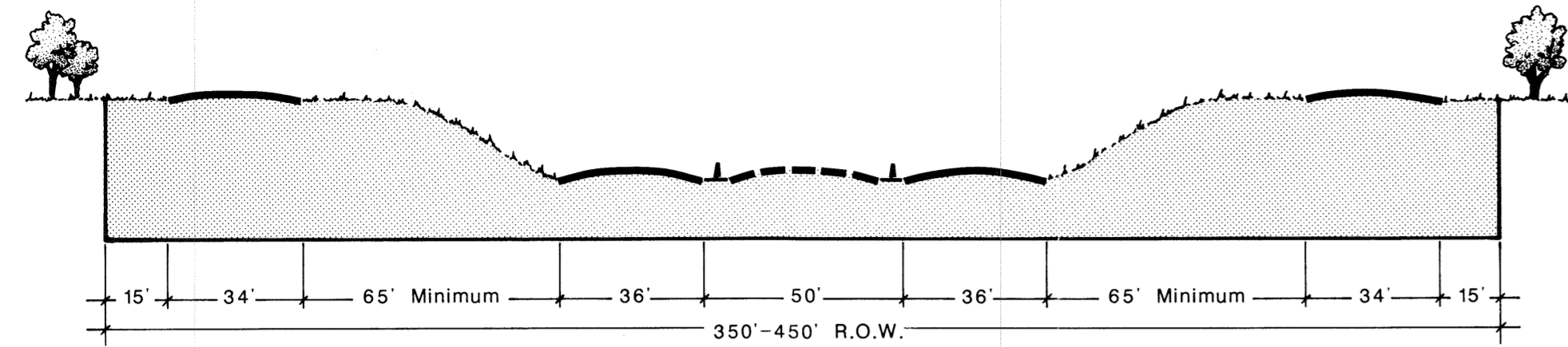
Type T (E6DF) Tollway - Regional
