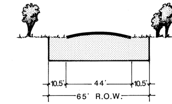
Type E (S4U) Secondary Thoroughfare
