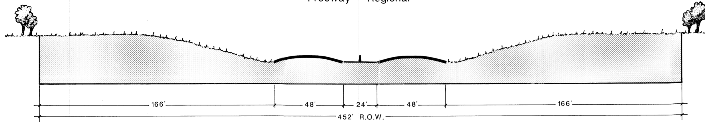
Type AA (E8DA) Freeway - Regional
