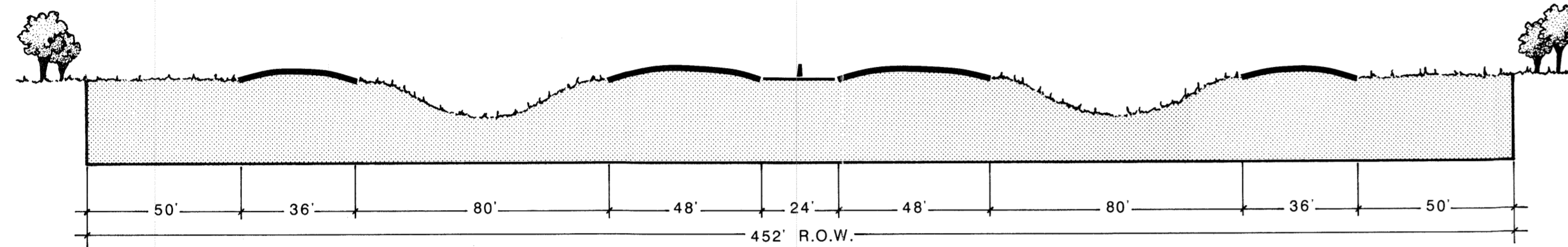
Type AA (E8DF) Freeway - Regional
