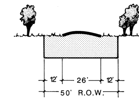
Type G (R2U) Residential/Local
