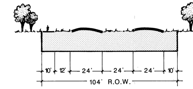
Type D (S4DI) Secondary Thoroughfare With Bike Path
