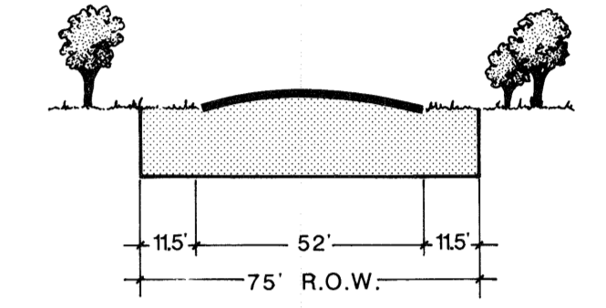
Type E (S4UIII) Secondary Thoroughfare With Bike Route
