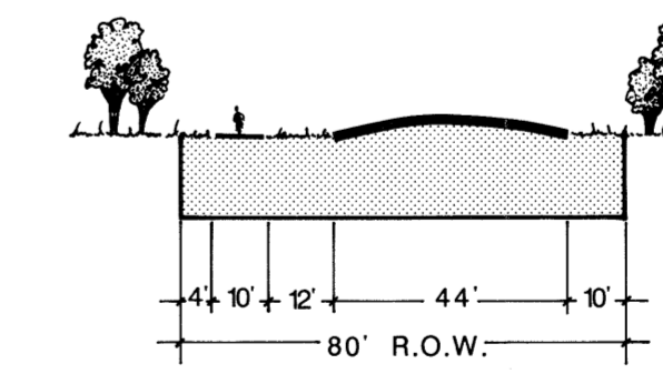
Type E (S4UI) Secondary Thoroughfare With Bike Path
