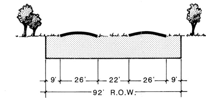
Type D (S4DIII) Secondary Thoroughfare With Bike Route
