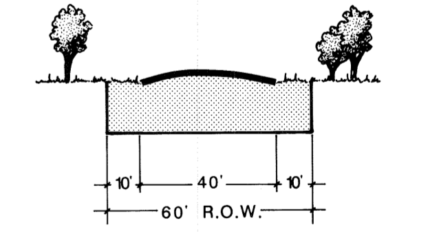
Type F (S2UIII) Collector With Bike Route
