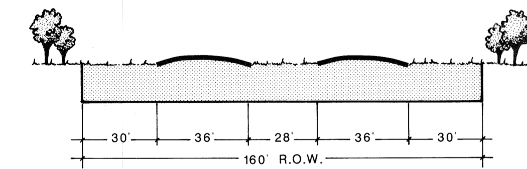
Type A (E6DA) Arterial - Regional Limited Access
