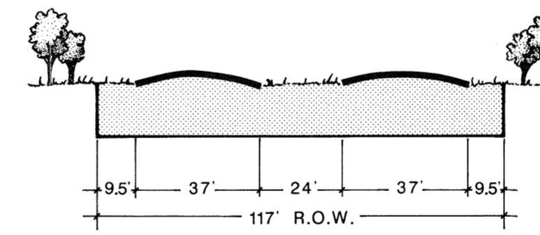
Type C (M6DIII) Major Thoroughfare With Bike Route
