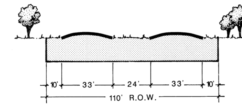
Type C (M6D) Major Thoroughfare
